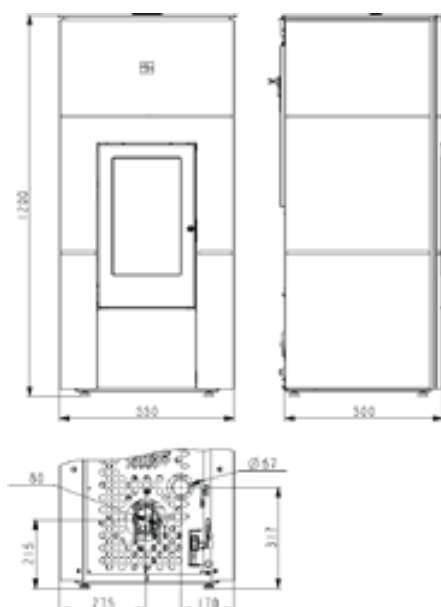
HSP 6 HELENA-C RLU perl-anthrazit, Keramik metal wet-aged 05 465 17 02 0000 EAN 90 027 42 47 5451
